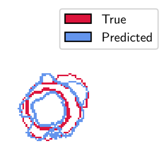
segmentations
